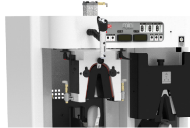
1 Hot - 1 Cold Station With Wipers (Flanging)
